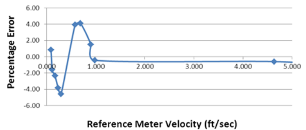
XGM868i/GF868 with T17 Transducers Low Flow % Error
